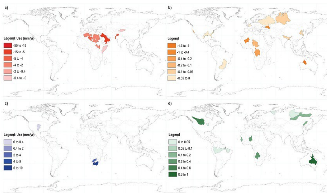
Figure 9. Renewable Groundwater Stress ratio derived from GRACE-based groundwater depletion. (a) Overstressed conditions and (c) human-dominated stress are shown as the rate of GRACE-based use assuming no available recharge (mm/yr). (b) Variable stressed conditions have a positive value of recharge and a negative value of use. (d) Unstressed systems have positive estimates of use and availability. The values are dimensionless in Figures 9b and 9d.
